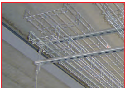
Multi-tiered cable basket
